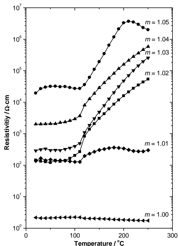
Fig. 5 Temperature dependence of total resistivity for ceramic compositions (Ba_{m-0.002}La_{0.002})TiO_3 with various (Ba+La)/Ti ratios m ranging between 1.00 and 1.05 sintered at 1573 K and p(O_2) = 10^{-9} MPa after subsequent reoxidation at 973 K in air for two hours.
