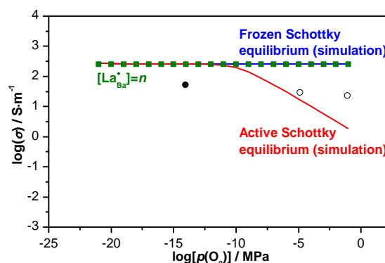
Fig. 6 Dependence of DC-conductivity for (Ba_{1.008}La_{0.002})TiO_3 at 1273 K from the partial pressure of oxygen p(O_2) . The black symbols represent experimentally determined values obtained after full equilibration (full symbol) and measured 24 hours after the adjustment of temperature and oxygen partial pressure (open symbols). The blue and red curves correspond to theoretical predictions, calculated from the concentration of free electrons n for the case that the Schottky reaction is assumed to be active (red curve) or frozen (blue curve). The green squared full symbols mark the conductivity expected for the supposed situation that the donor concentration of 0.2 mol.-% of La is fully incorporated into the perovskite lattice.
