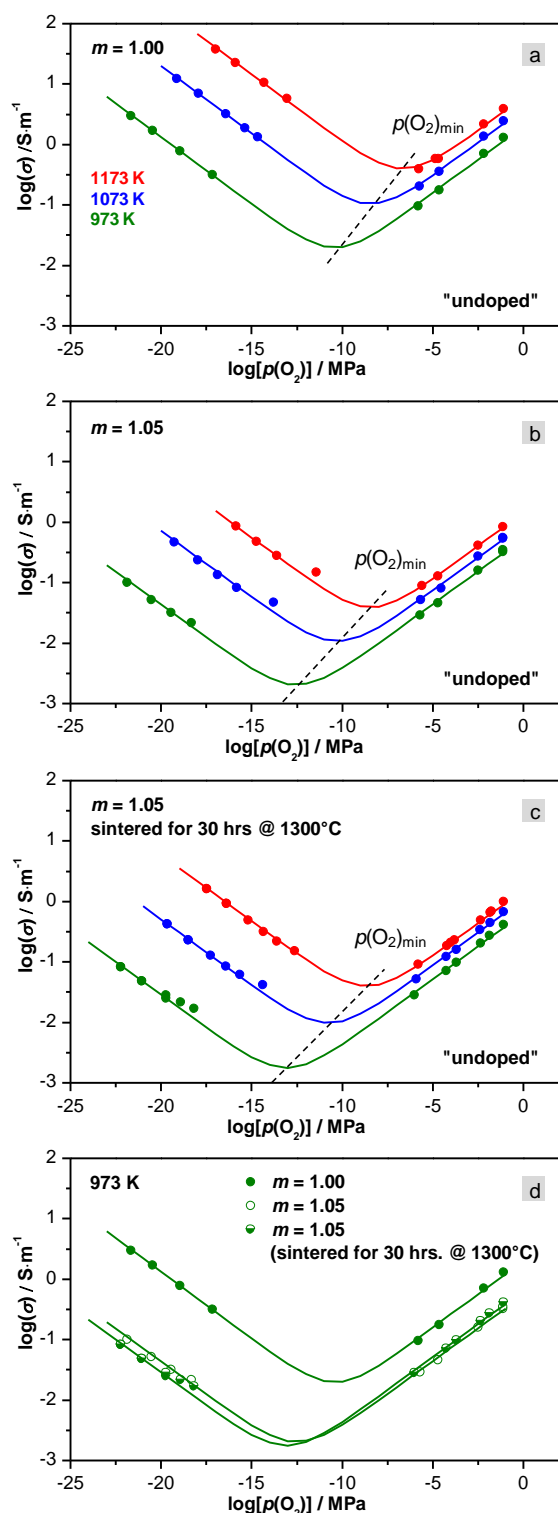
Fig. 13 Modified Kröger-Vink diagrams for (a) stoichiometric ( m = 1 ) and (b) hyper-stoichiometric ( m = 1.05 ) nominally undoped \text{Ba}_m\text{TiO}_{3+m} sintered at 1350 °C for two hours. The case of hyper-stoichiometric \text{Ba}_{1.05}\text{TiO}_{3.05} that was additionally soaked for 30 hours at 1300 °C after sintering is shown in (c) and (d) represents a comparison of the conductivity in dependence of oxygen partial pressure p(\text{O}_2) of all three materials at 973 K.
